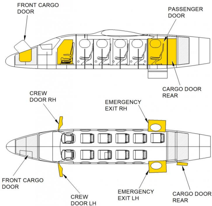
Figure 7-16 - Tecnam P2012 Doors Layout
